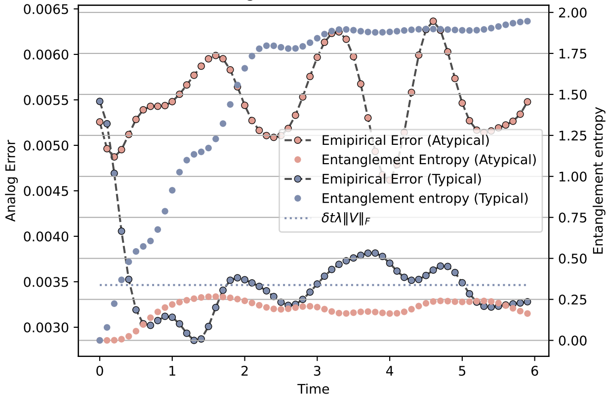
QIMF, one segment evolution with disorder
